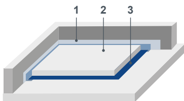
1. Foam Expansion Strip with film 2. Screed 3. Bogus paper
