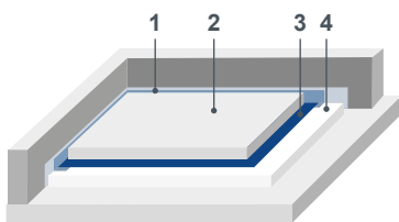
1. Foam Expansion Strip with film 2. Screed 3. Bogus paper 4. Footfall sound insulation and thermal insulation
