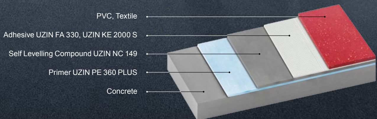
Example Construction
