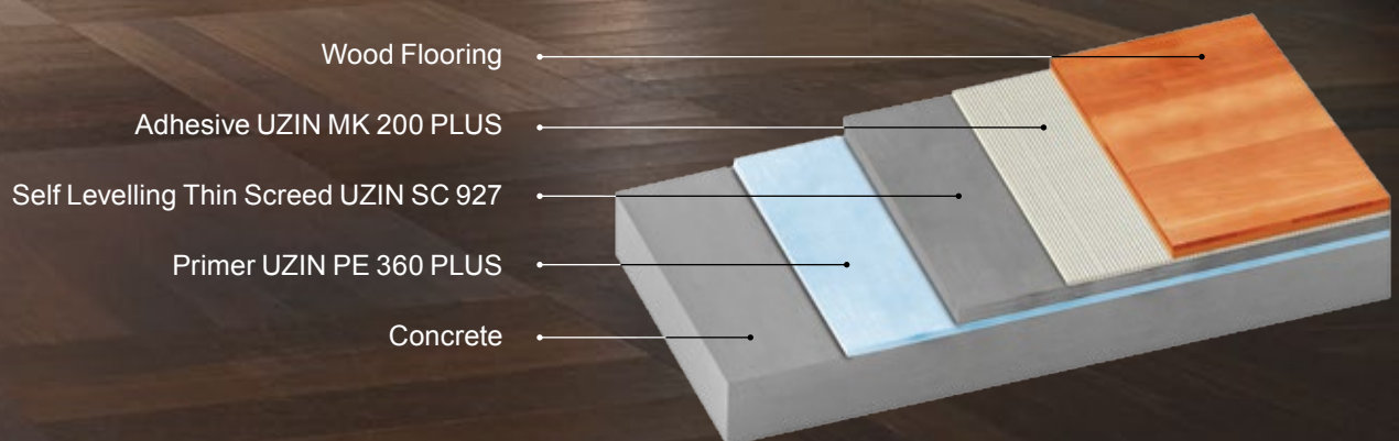
Example Construction
