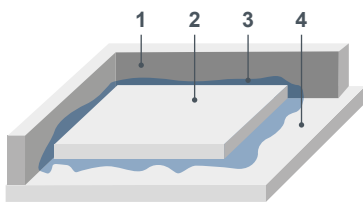
1. Wall 2. Screed 3. Primer 4. Subfloor (e.g. concrete)
