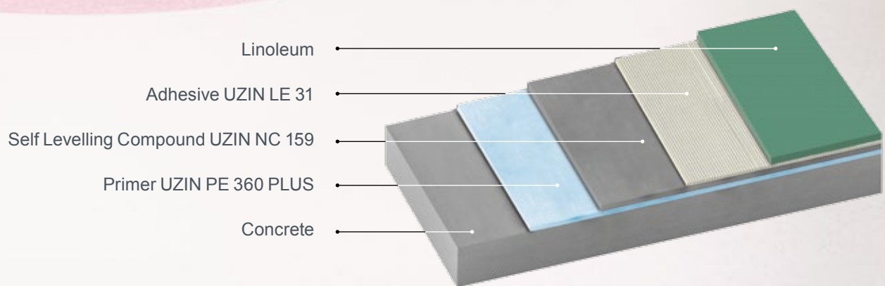
Example Construction
